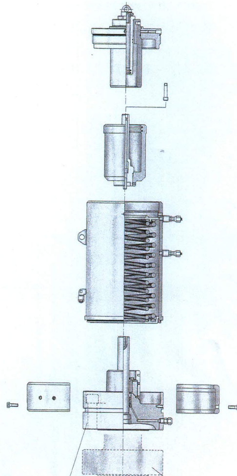
"OFS/SD" DIAPHRAGM ACTUATOR
